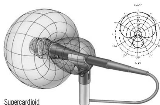
Cardioid (unidirectional)
